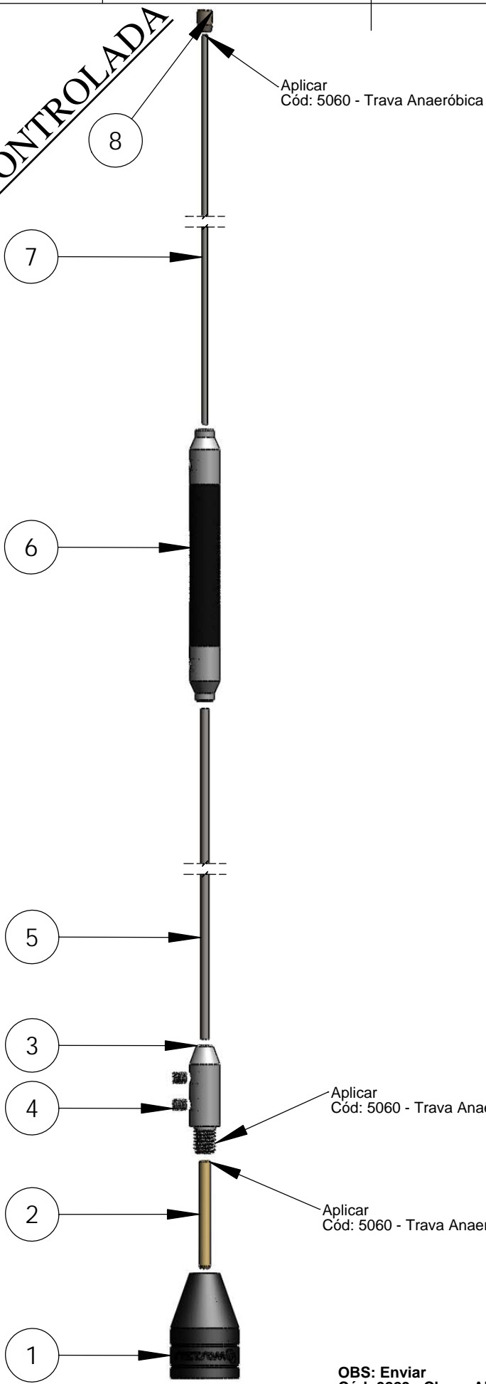
VISTA EXPLODIDA
