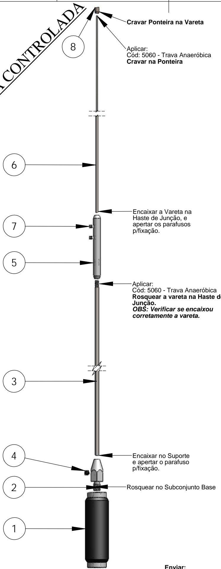
VISTA EXPLODIDA
